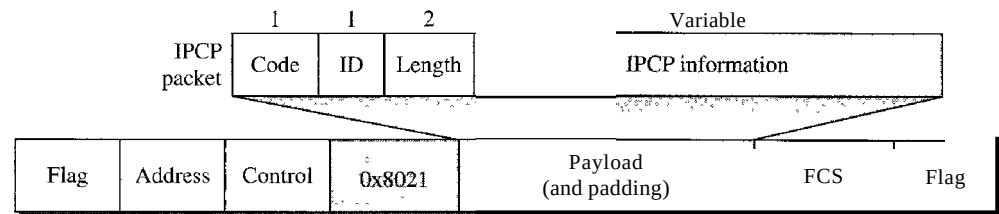
Figure 11.38 fPCP packet encapsulated in PPP frame
