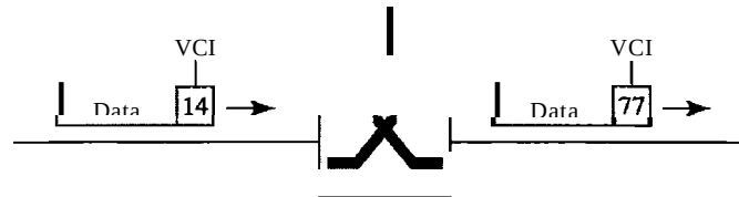
Figure 8.11 Virtual-circuit identifier
