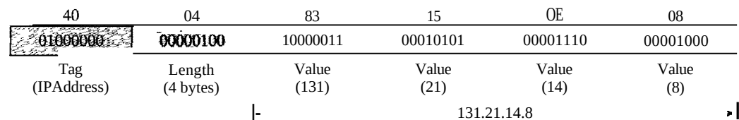
Figure 28.14 Example 28.4, IPAddress 131.21.14.8
