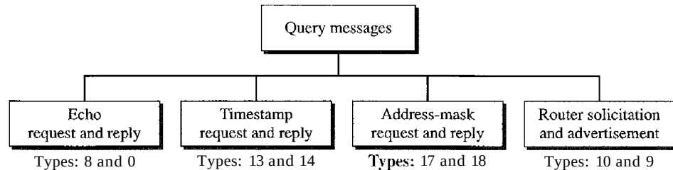
Figure 21.12 Query messages
