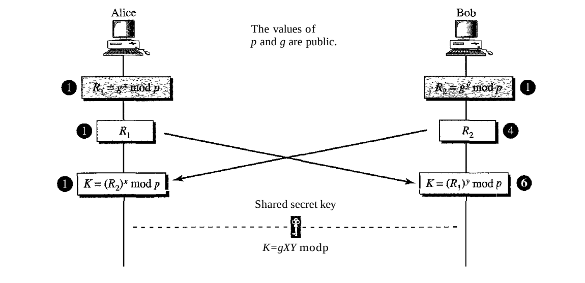
Figure 30.26 Diffie-Hellman method
