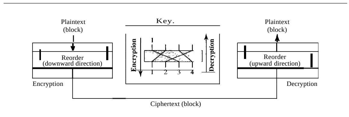
Figure 30.8 Transposition cipher
